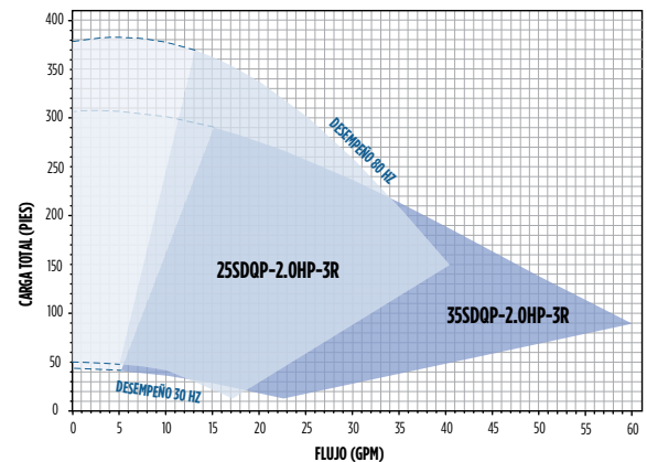
SUBDRIVE 20
