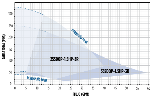
SUBDRIVE 15
