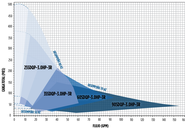
SUBDRIVE 30
